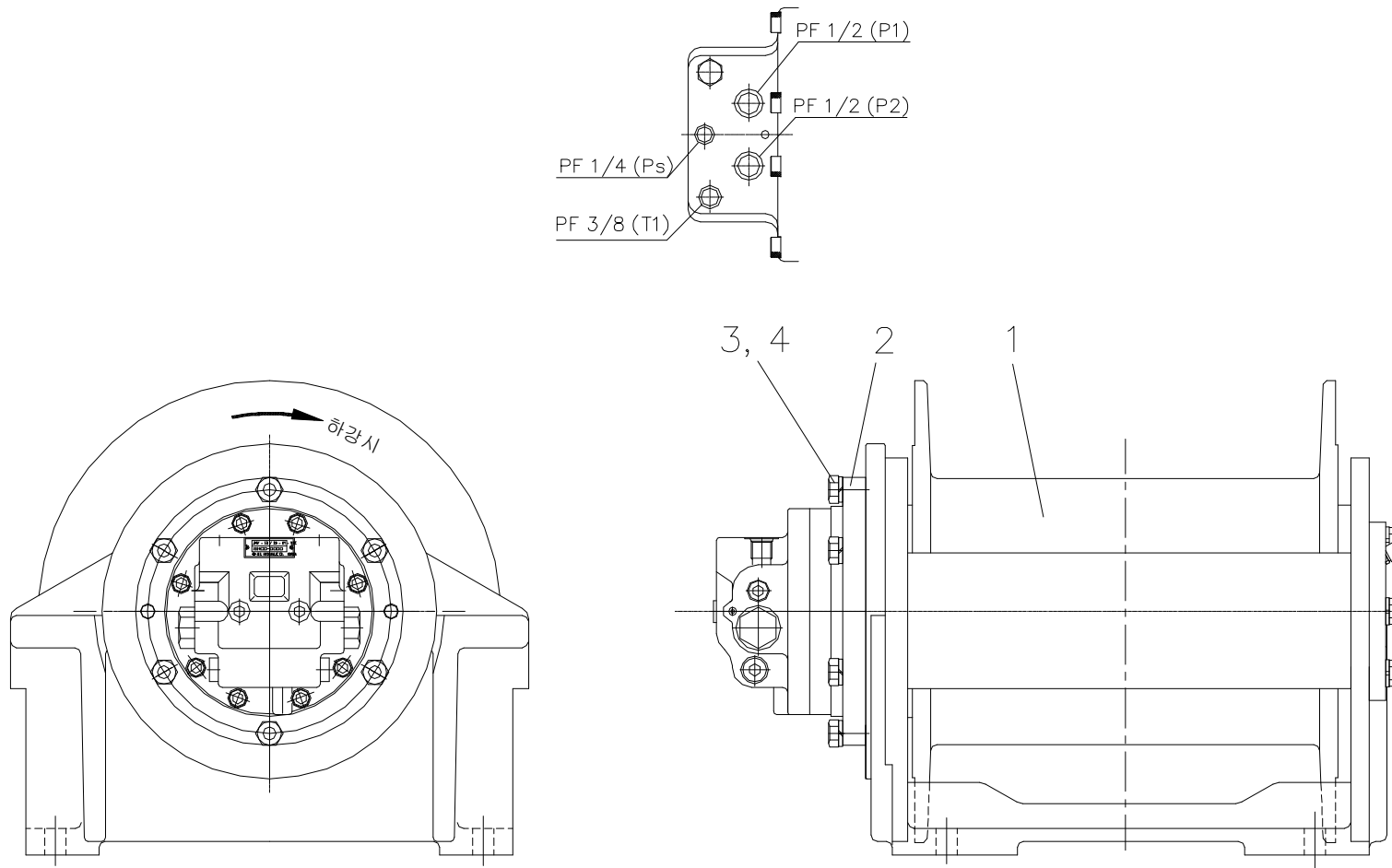
Fig. 2-1 SCS1015LSuper 2 SPEED WINCH ASS'Y
