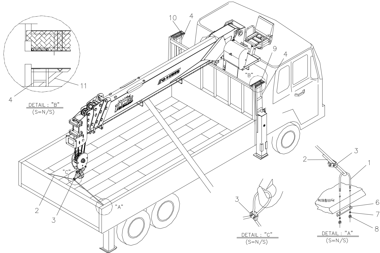
Fig. 10-5 SCS1015LSuper LOADING BOX PART
