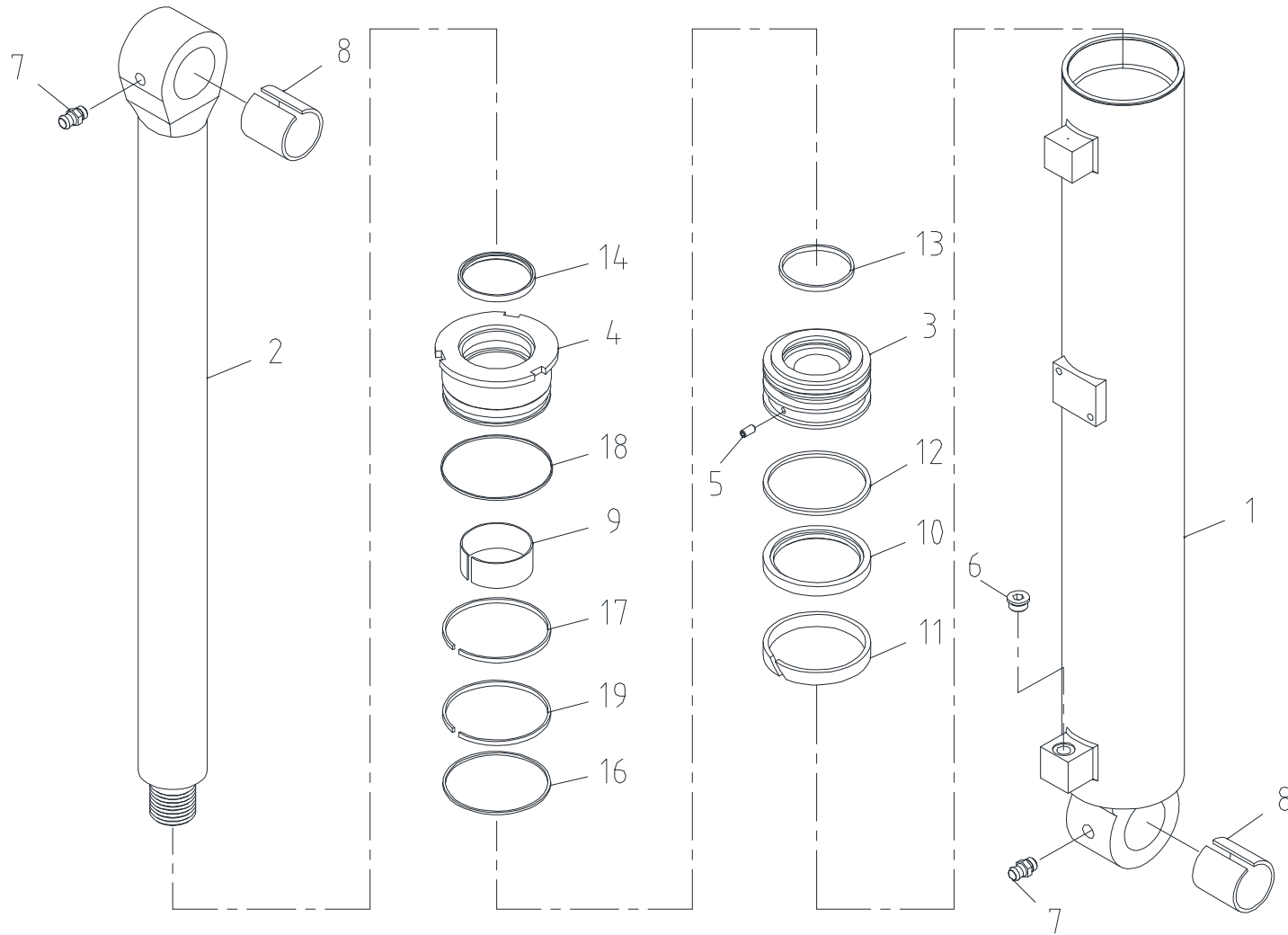
Fig. 2-3 SCS1015LSuper DERRICK CYL' ASS'Y
