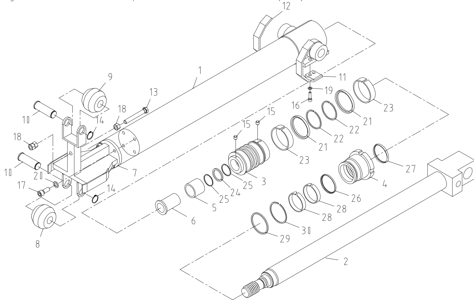
Fig. 1-1-2 SCS1015LSuper TELESCOPIC CYLINDER (2nd) ASS'Y
