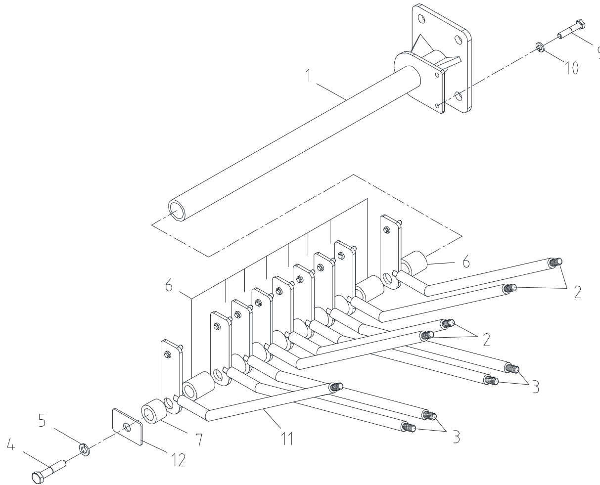
Fig. 3-2-2 SCS1015LSuper LEVER STAND SET
