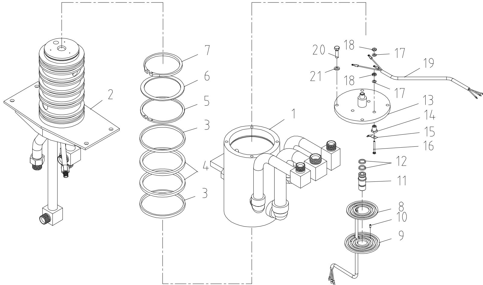
Fig. 3-1 SCS1015LSuper ROTARY JOINT ASS'Y
