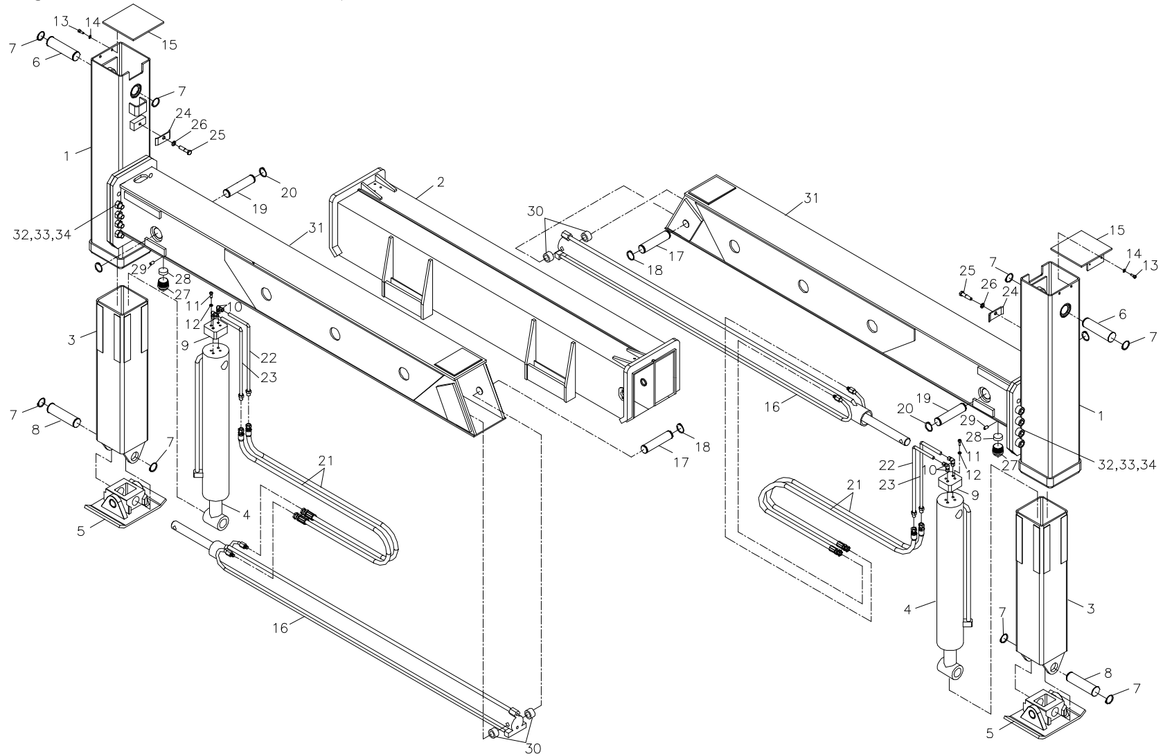
Fig. 10-2-1 SCS1015LSuper REAR OUTRIGGER ASS'Y
