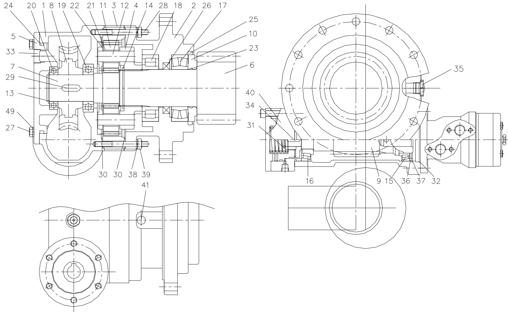
Fig. 2-2 SCS1015LSuper SWING GEAR ASS'Y
