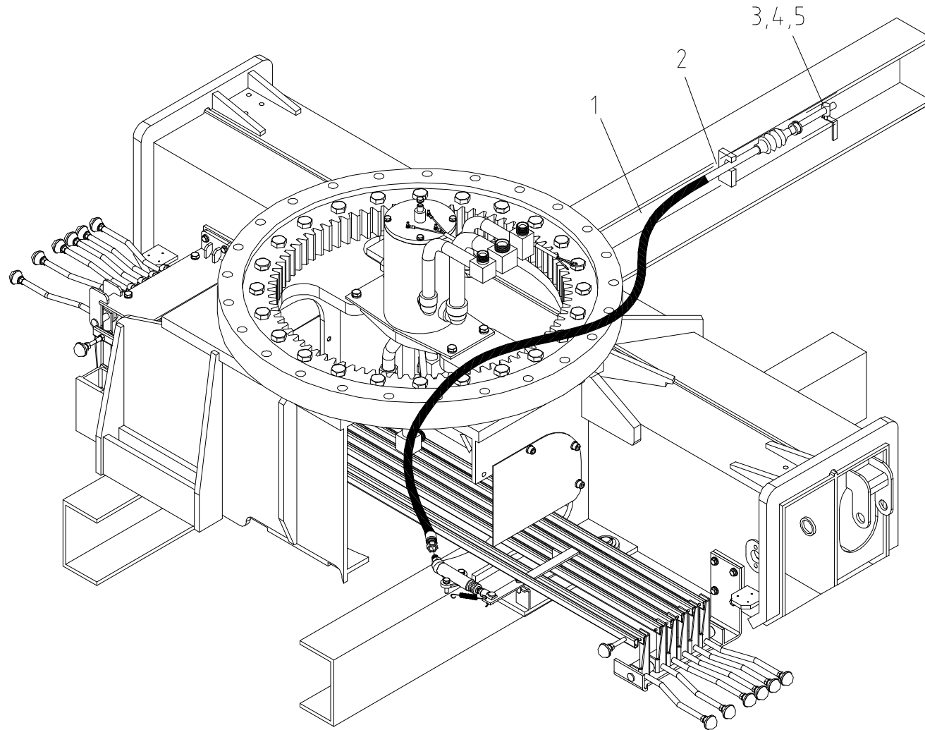
Fig. 10-3 SCS1015LSuper ACC'L SYSTEM PART
