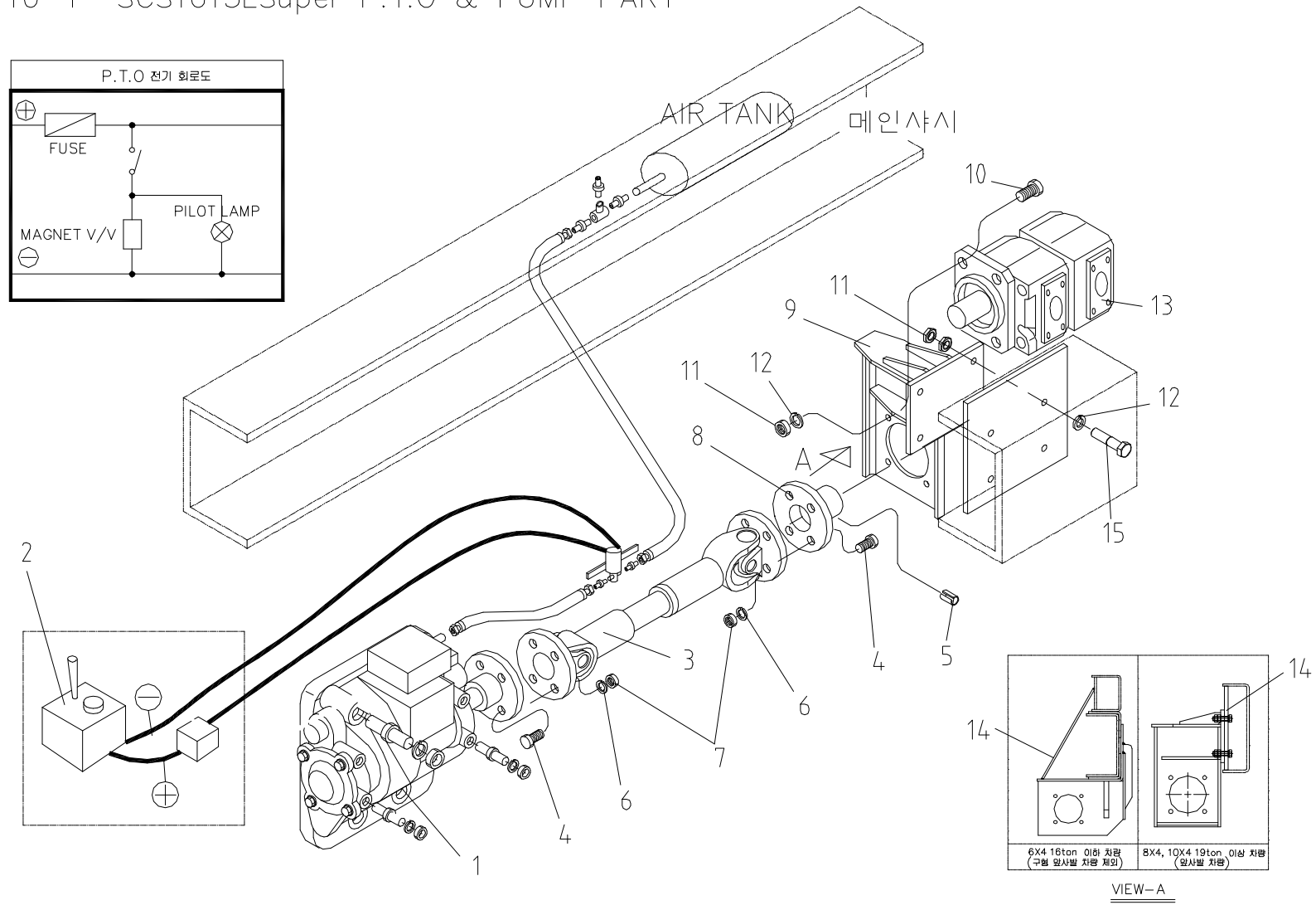
Fig. 10-1 SCS1015LSuper P.T.O &amp; PUMP PART
